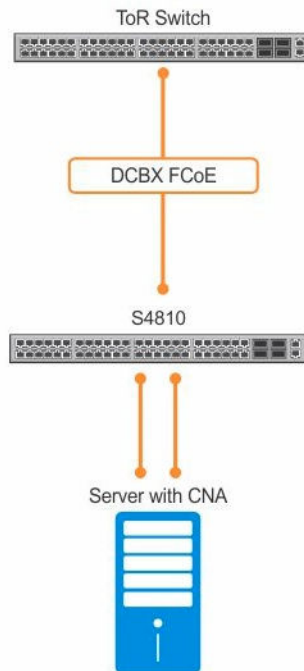
Figure 35. Configuration Example: FIP Snooping on a Switch
